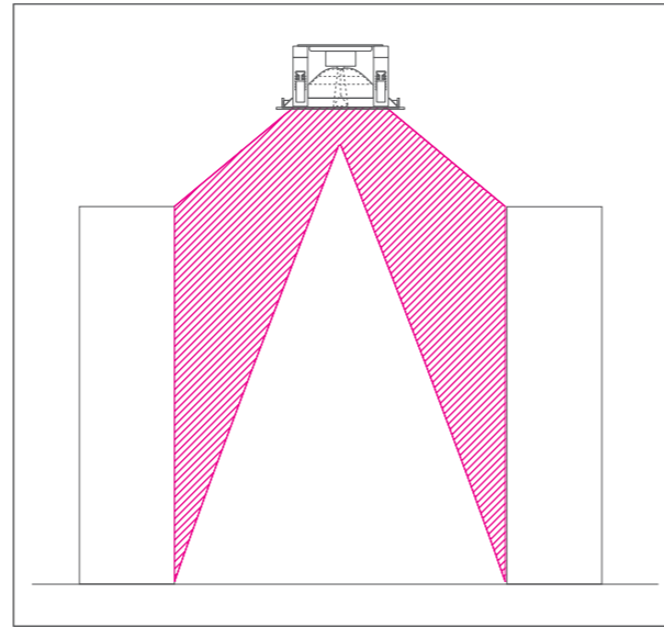
REON DA MAX • LIGHT CHARACTERISTICS • FRONT VIEW
