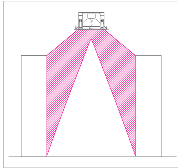
REON DA • LIGHT CHARACTERISTICS • FRONT VIEW
