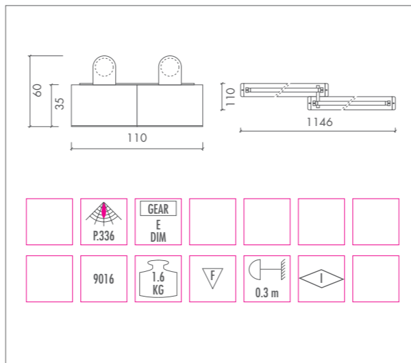
CROSS-LINE • 2xT5 13W / 14W / 22W / 24W • G5
