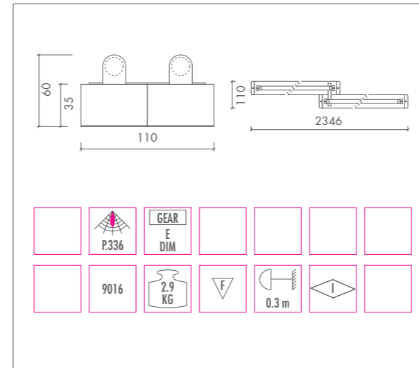
CROSS-LINE • 2xT5 25W / 28W / 50W / 54W • G5
