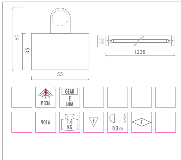
CROSS-LINE • 1xT5 25W / 28W / 50W / 54W • G5
