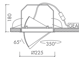
TOCLA Z SQUARE • RGB LED 12W
